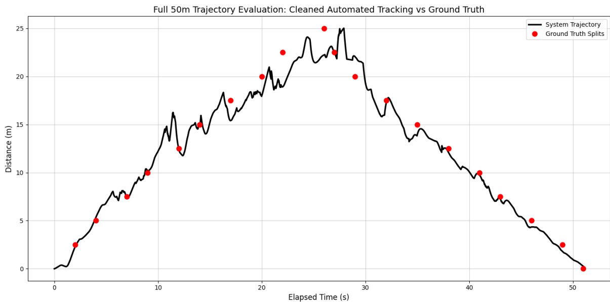
Figure 5.2 Full 50 m trajectory evaluation: system trajectory (black line) versus manually recorded ground truth split times (red points). The y-axis represents the distance from the origin (start wall). The swimmer travels from 0 m to 25 m (outbound) and returns to 0 m.
