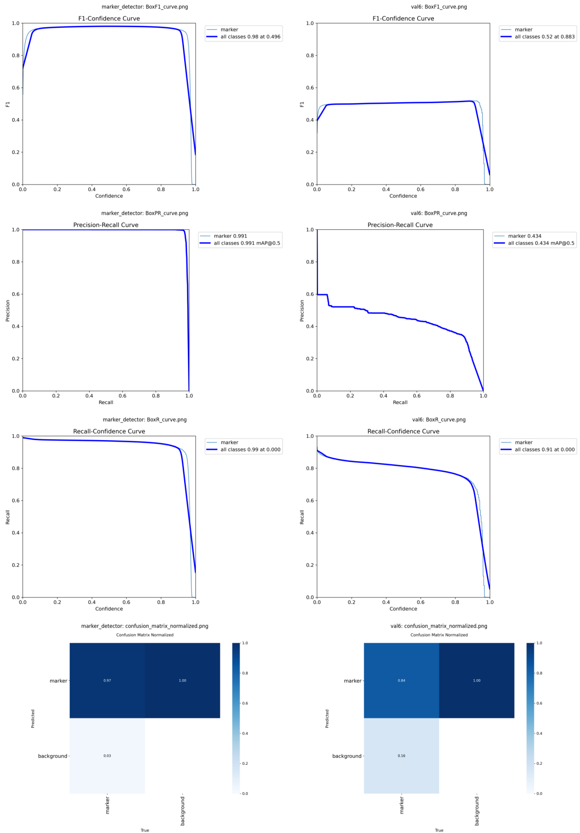
Figure 5.1 Comparison of marker detection accuracy. Left: Inference on test frames from the training video, showing high confidence and precision. Right: Inference on an unseen video from the same pool.
